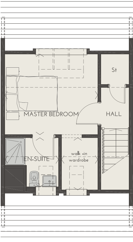
Legend: W - built-in wardrobe St - store
